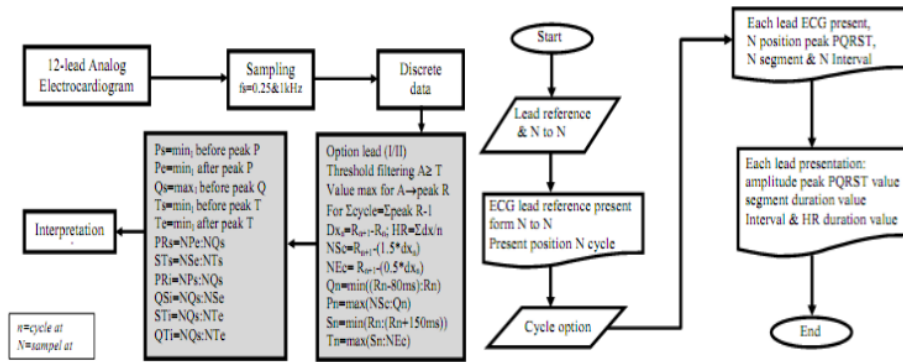
Figure 8. PQRST Algorithm and flowchart
